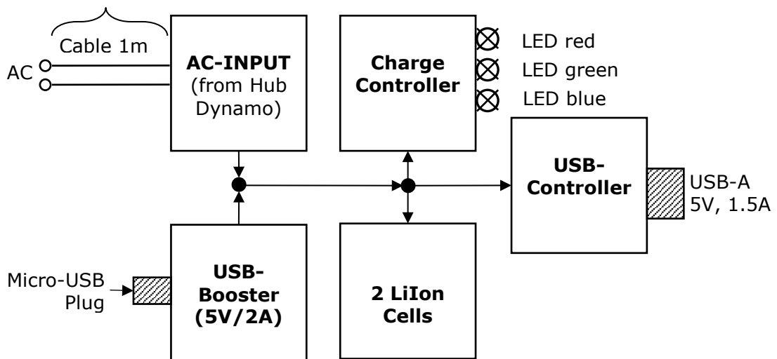
Fig 2: Harvester Functional Diagram
